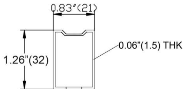
END SECTION VIEW
