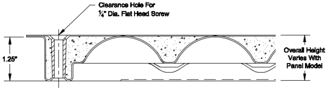
PARTIAL SECTION VIEW
