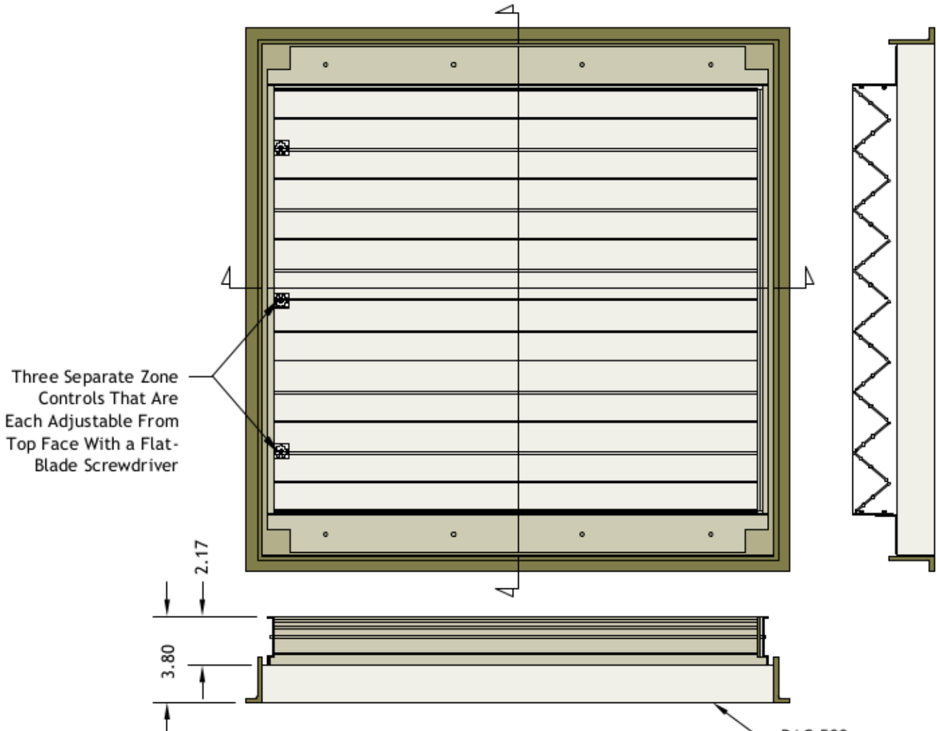
DAG 500 Directional Air Flow Grate 24" or 600mm Size
